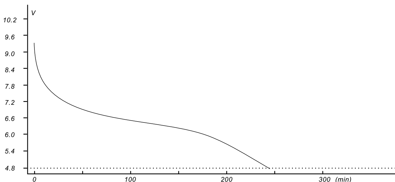
Discharge Load 180 \Omega (24h/1d)
